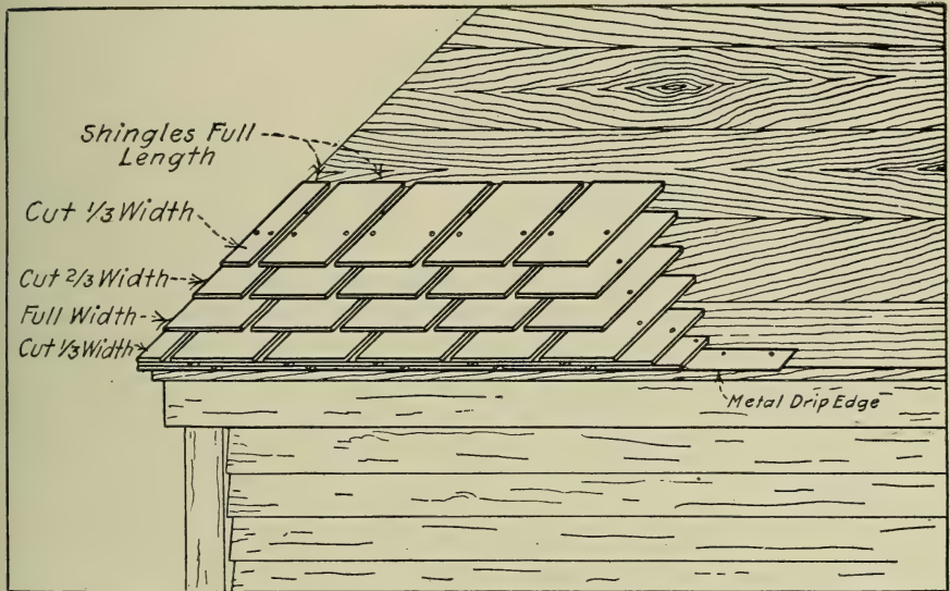
FIG. 147.—Laying Individual Shingles.
